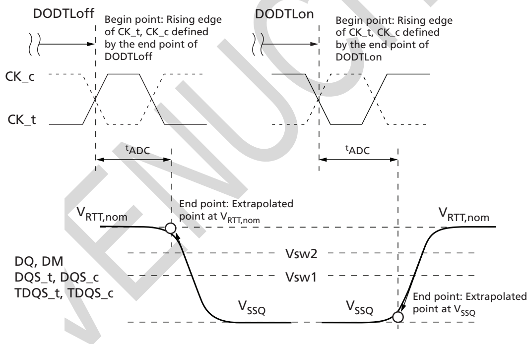
Figure 241: t_{ADC} Definition with Direct ODT Control
