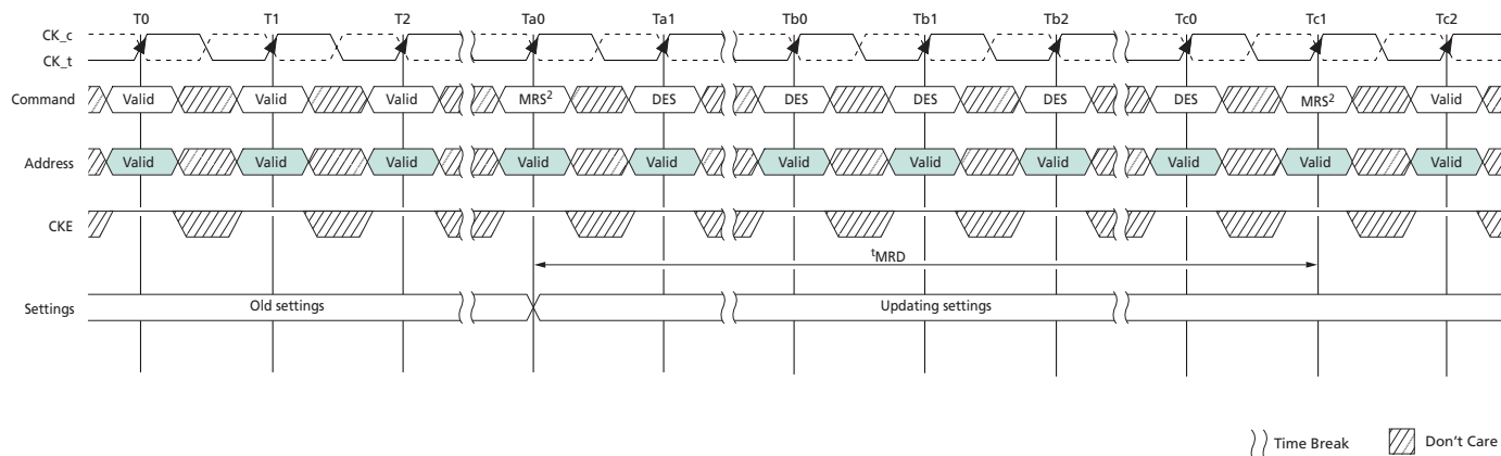
Figure 16: t^{\text{MRD}} Timing
