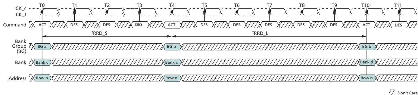
Figure 121: t_{RRD} Timing
